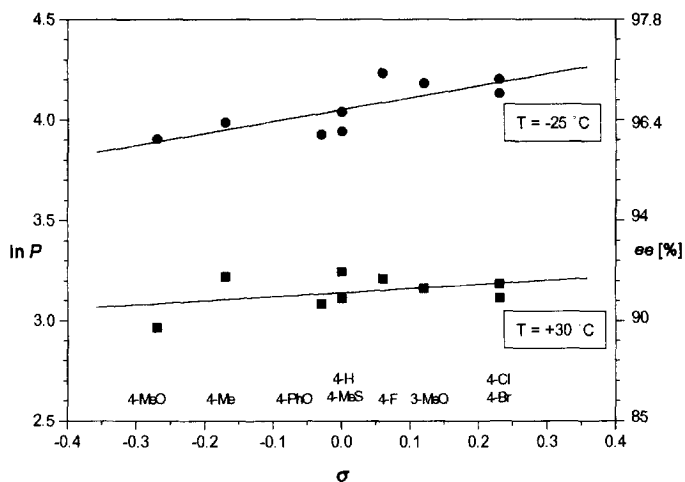
Figure 7. Plot of the \ln P -values (at T = -25\text{ }^\circ\text{C} and +30\text{ }^\circ\text{C} ) achievable with each substituent X vs. the corresponding Hammett constants \sigma .
