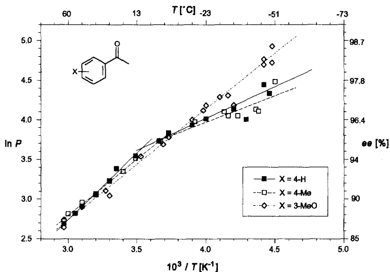
Figure 5. Eyring diagram for the reduction of the 4-X-acetophenones ( X = \text{H}, \text{Me} ) and of 3-MeO-acetophenone with 1.
