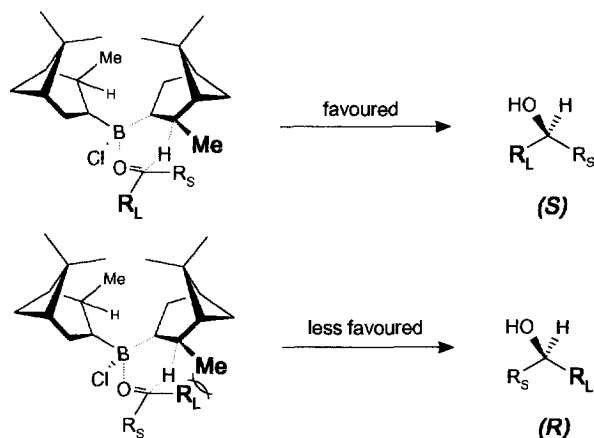
Figure 2: One-step transition state model for the asymmetric reduction of ketones with (-)-Ipc 2 BCl proposed by Brown et al. 1
