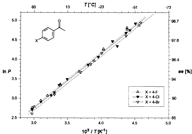
Figure 4. Eyring diagram for the reduction of the 4-halogen-acetophenones with 1.
