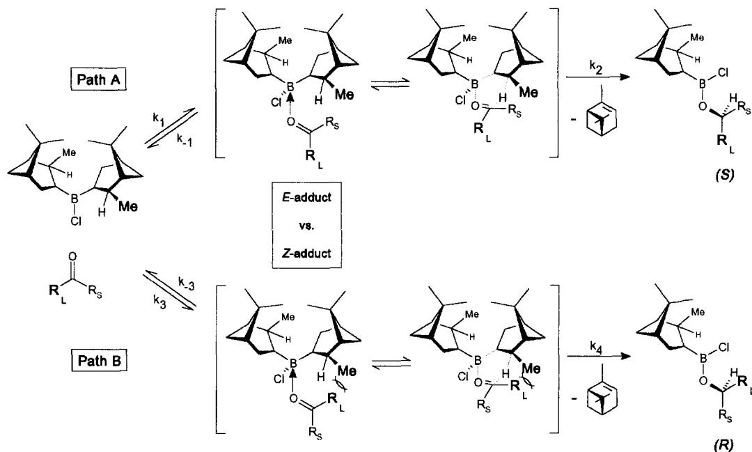
Figure 8. Tentative model of the partial steps in asymmetric reductions of ketones with (-)-Ipc 2 BCl being relevant for stereoselection (here: R L = Ph, R S = Me).
