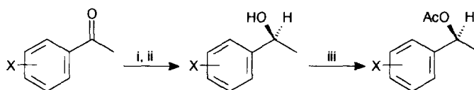
Figure 3. Standard procedure: i. 1.3 eq. 1 , THF, x °C; ii. H 2 O 2 /NaHCO 3 or diethanolamine; iii. pyridine, acetylchloride, Et 2 O, room temperature (except in the case of X = 4-MeS, where propionylchloride was used).
