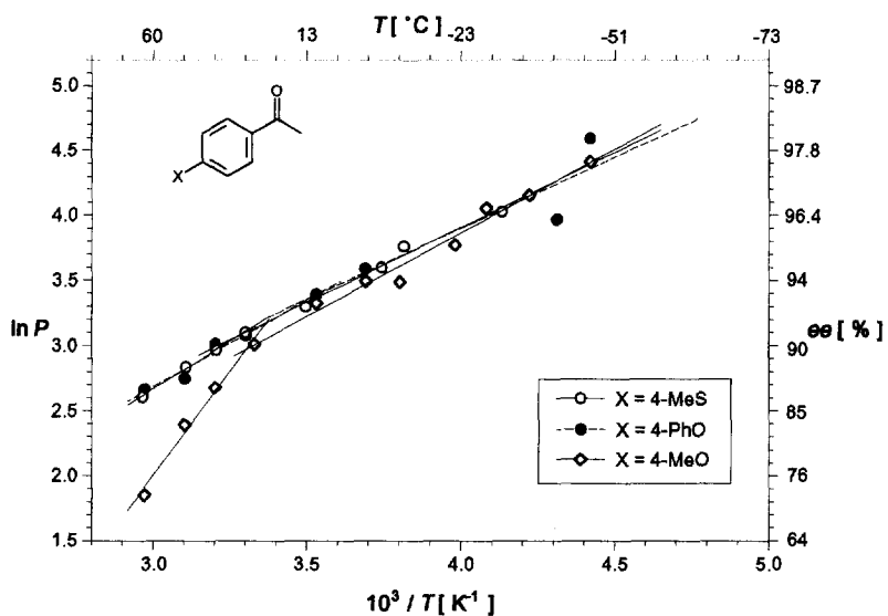
Figure 6. Eyring diagram for the reduction of ether- and thioether-acetophenones ( X = 4\text{-MeO}, 4\text{-PhO}, 4\text{-MeS} ) with 1.
